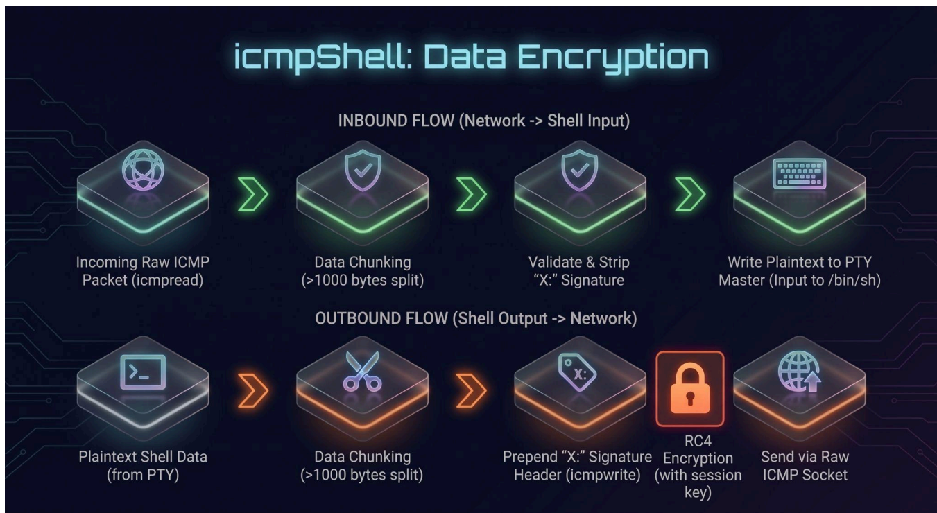
Figure 40: icmpShell data encryption
