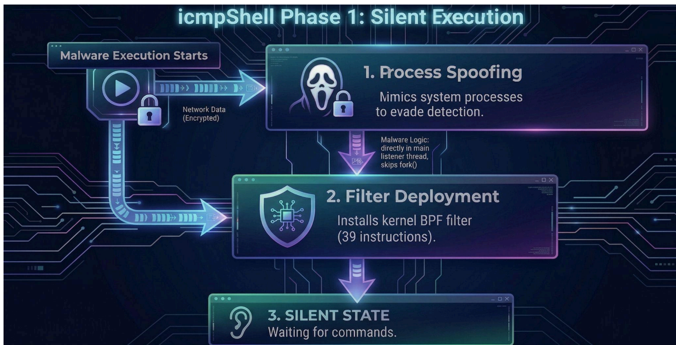
Figure 27: icmpShell Phase1 performing process spoofing and installing BPF filter
