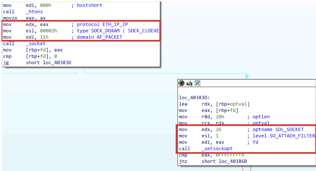
Figure 6: socket creation and filter attachment flags
