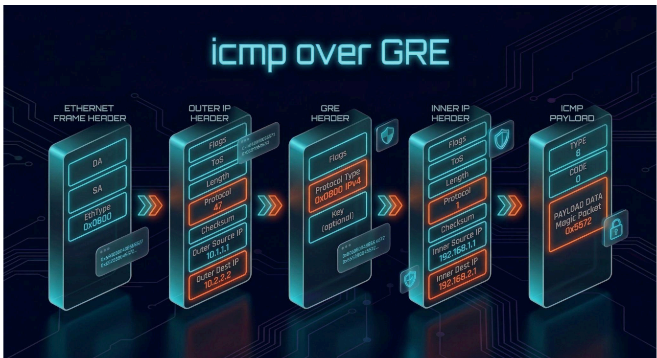
Figure 10: ICMP over GRE tunnel
